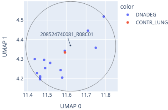
Close-up of UMAP for 208524740081_R08C01 reference: AllIDATv2_20210804_HPAP_Sarc.xlsx (19967 cases), 0 CpGs
