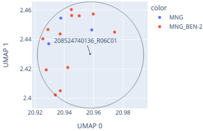
Close-up of UMAP for 208524740136_R06C01 reference: AllIDATv2_20210804_HPAP_Sarc.xlsx (19967 cases), 0 CpGs
