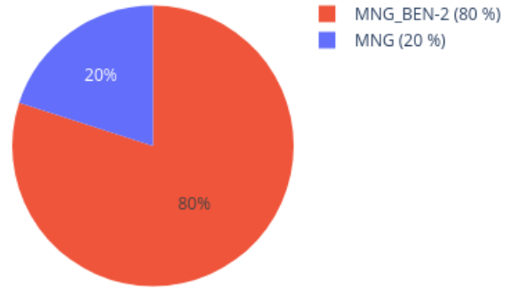
Neighbors in UMAP for 208524740136_R06C01 reference: AllIDATv2_20210804_HPAP_Sarc.xlsx (19967 cases), 0 CpGs
