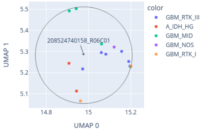
Close-up of UMAP for 208524740158_R06C01 reference: AllIDATv2_20210804_HPAP_Sarc.xlsx (19967 cases), 0 CpGs
