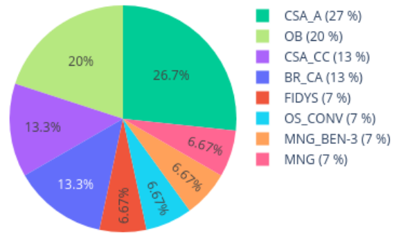
Neighbors in UMAP for 208524740158_R08C01 reference: AllIDATv2_20210804_HPAP_Sarc.xlsx (19967 cases), 0 CpGs
