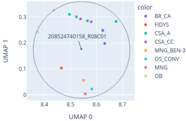
Close-up of UMAP for 208524740158_R08C01 reference: AllIDATv2_20210804_HPAP_Sarc.xlsx (19967 cases), 0 CpGs
