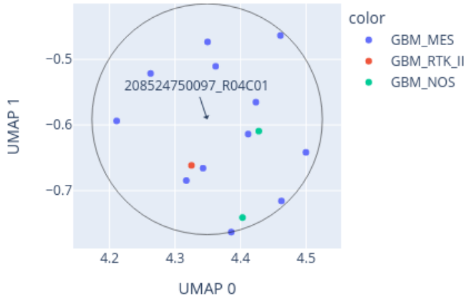
Close-up of UMAP for 208524750097_R04C01 reference: AllIDATv2_20210804_HPAP_Sarc.xlsx (19967 cases), 0 CpGs
