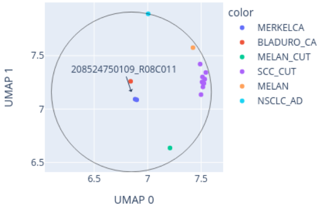
Close-up of UMAP for 208524750109_R08C011 reference: AllIDATv2_20210804_HPAP_Sarc.xlsx (19967 cases), 0 CpGs
