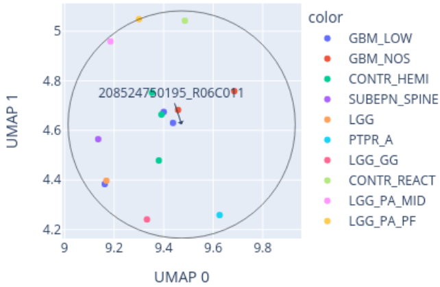
Close-up of UMAP for 208524750195_R06C011 reference: AllIDATv2_20210804_HPAP_Sarc.xlsx (19967 cases), 0 CpGs
