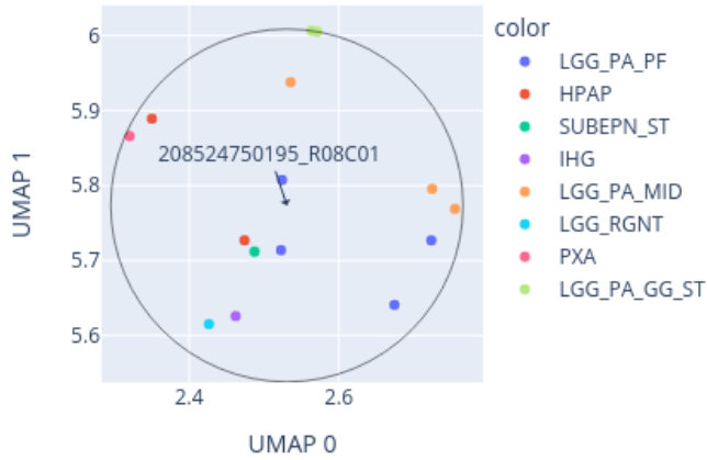
Close-up of UMAP for 208524750195_R08C01 reference: AllIDATv2_20210804_HPAP_Sarc.xlsx (19967 cases), 0 CpGs
