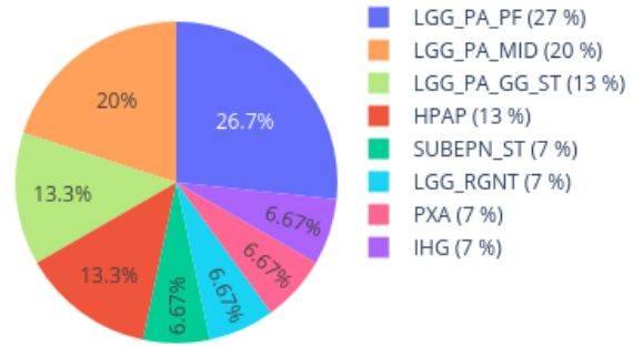
Neighbors in UMAP for 208524750195_R08C01 reference: AllIDATv2_20210804_HPAP_Sarc.xlsx (19967 cases), 0 CpGs
