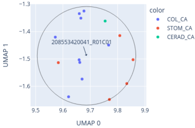
Close-up of UMAP for 208553420041_R01C01 reference: AllIDATv2_20210804_HPAP_Sarc.xlsx (19967 cases), 0 CpGs
