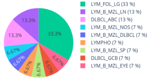
Neighbors in UMAP for 208553420089_R07C011 reference: AllIDATv2_20210804_HPAP_Sarc.xlsx (19967 cases), 0 CpGs
