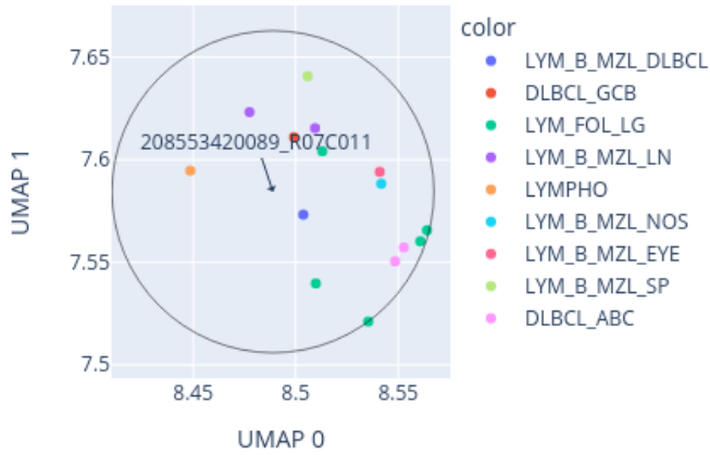
Close-up of UMAP for 208553420089_R07C011 reference: AllIDATv2_20210804_HPAP_Sarc.xlsx (19967 cases), 0 CpGs
