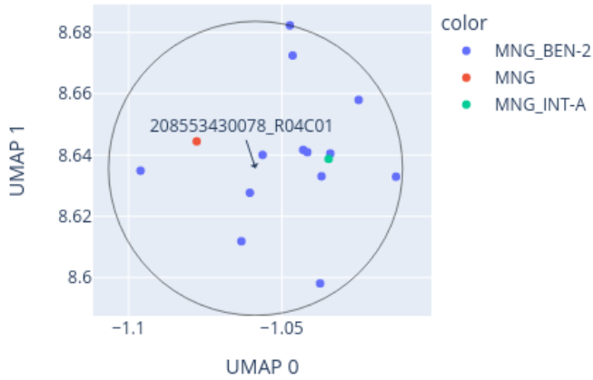
Close-up of UMAP for 208553430078_R04C01 reference: AllIDATv2_20210804_HPAP_Sarc.xlsx (19967 cases), 0 CpGs
