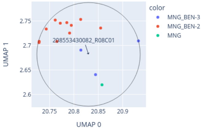
Close-up of UMAP for 208553430082_R08C01 reference: AllIDATv2_20210804_HPAP_Sarc.xlsx (19967 cases), 0 CpGs
