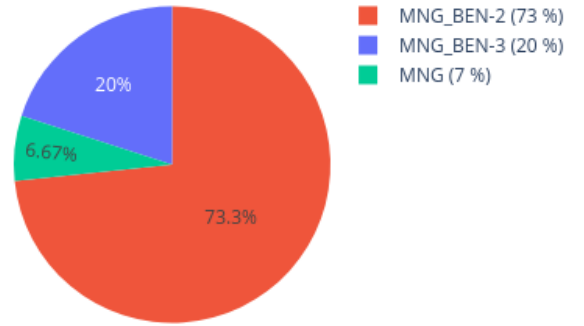
Neighbors in UMAP for 208553430082_R08C01 reference: AllIDATv2_20210804_HPAP_Sarc.xlsx (19967 cases), 0 CpGs
