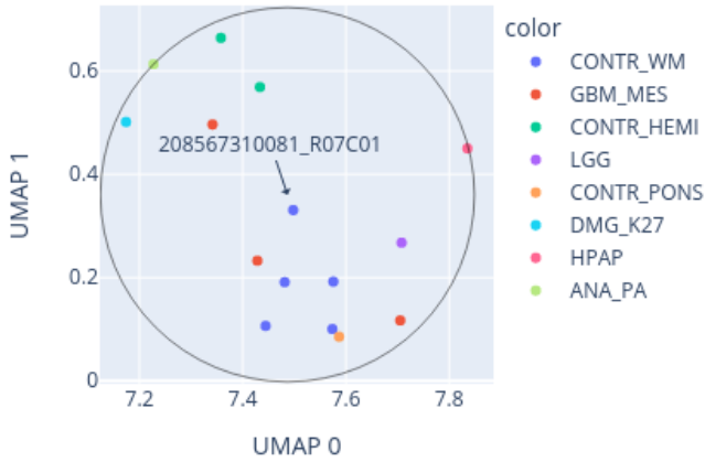
Close-up of UMAP for 208567310081_R07C01 reference: AllIDATv2_20210804_HPAP_Sarc.xlsx (19967 cases), 0 CpGs
