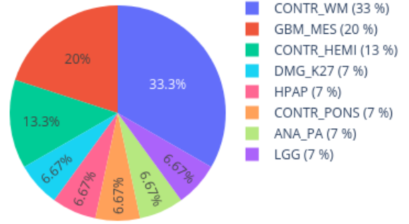
Neighbors in UMAP for 208567310081_R07C01 reference: AllIDATv2_20210804_HPAP_Sarc.xlsx (19967 cases), 0 CpGs
