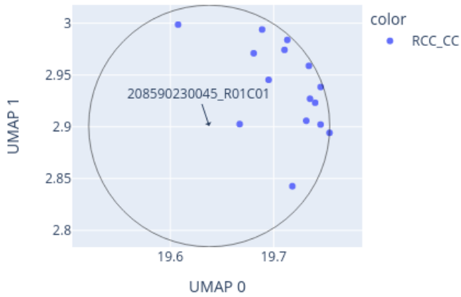
Close-up of UMAP for 208590230045_R01C01 reference: AllIDATv2_20210804_HPAP_Sarc.xlsx (19967 cases), 0 CpGs
