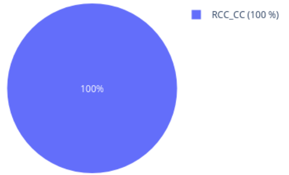
Neighbors in UMAP for 208590230045_R01C01 reference: AllIDATv2_20210804_HPAP_Sarc.xlsx (19967 cases), 0 CpGs
