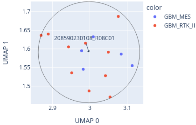
Close-up of UMAP for 208590230108_R08C01 reference: AllIDATv2_20210804_HPAP_Sarc.xlsx (19967 cases), 0 CpGs
