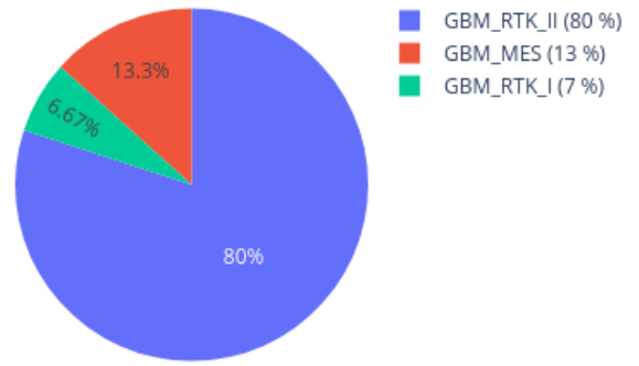
Neighbors in UMAP for 208590230151_R06C01 reference: AllIDATv2_20210804_HPAP_Sarc.xlsx (19967 cases), 0 CpGs
