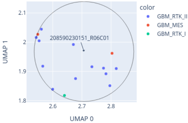
Close-up of UMAP for 208590230151_R06C01 reference: AllIDATv2_20210804_HPAP_Sarc.xlsx (19967 cases), 0 CpGs
