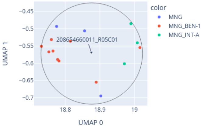
Close-up of UMAP for 208654660011_R05C01 reference: AllIDATv2_20210804_HPAP_Sarc.xlsx (19967 cases), 0 CpGs
