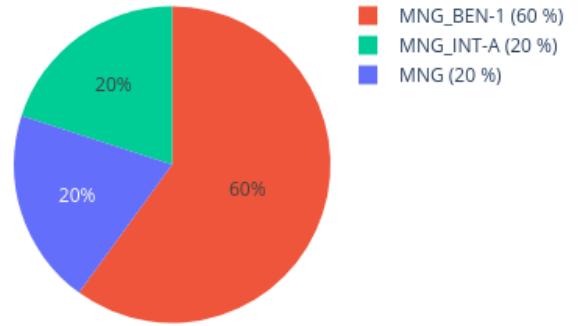
Neighbors in UMAP for 208654660011_R05C01 reference: AllIDATv2_20210804_HPAP_Sarc.xlsx (19967 cases), 0 CpGs
