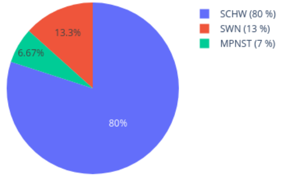
Neighbors in UMAP for 208654660037_R06C01 reference: AllIDATv2_20210804_HPAP_Sarc.xlsx (19967 cases), 0 CpGs
