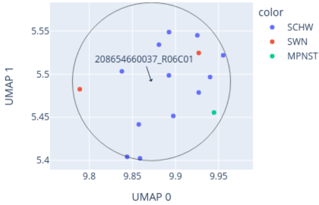
Close-up of UMAP for 208654660037_R06C01 reference: AllIDATv2_20210804_HPAP_Sarc.xlsx (19967 cases), 0 CpGs
