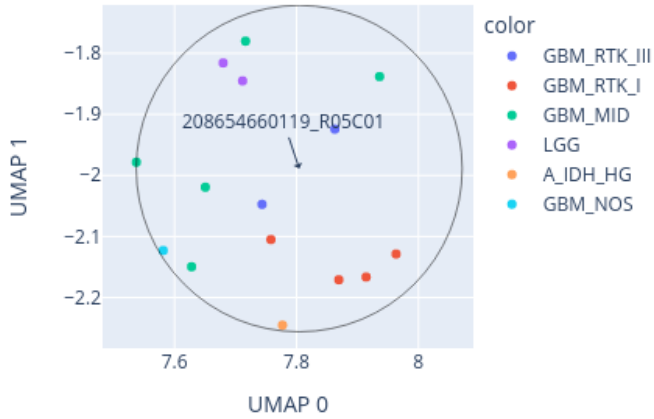
Close-up of UMAP for 208654660119_R05C01 reference: AllIDATv2_20210804_HPAP_Sarc.xlsx (19967 cases), 0 CpGs
