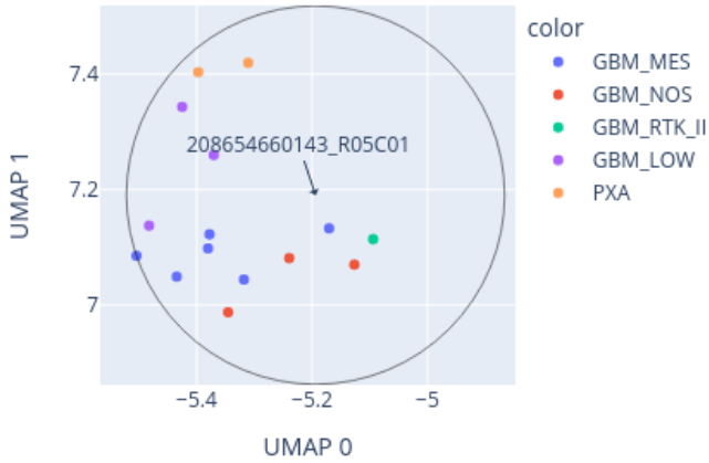
Close-up of UMAP for 208654660143_R05C01 reference: AllIDATv2_20210804_HPAP_Sarc.xlsx (19967 cases), 0 CpGs
