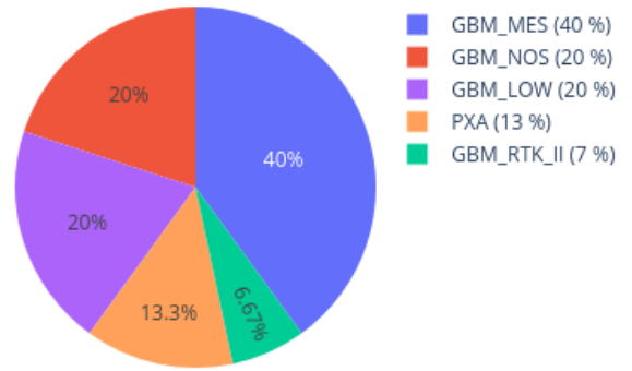
Neighbors in UMAP for 208654660143_R05C01 reference: AllIDATv2_20210804_HPAP_Sarc.xlsx (19967 cases), 0 CpGs
