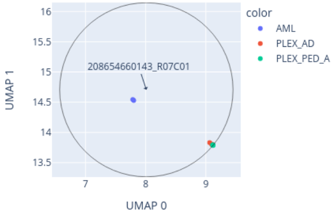
Close-up of UMAP for 208654660143_R07C01 reference: AllIDATv2_20210804_HPAP_Sarc.xlsx (19967 cases), 0 CpGs
