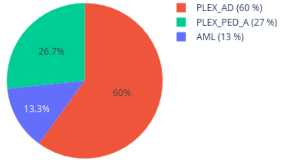
Neighbors in UMAP for 208654660143_R07C01 reference: AllIDATv2_20210804_HPAP_Sarc.xlsx (19967 cases), 0 CpGs
