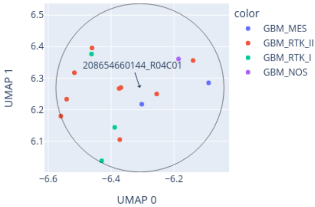
Close-up of UMAP for 208654660144_R04C01 reference: AllIDATv2_20210804_HPAP_Sarc.xlsx (19967 cases), 0 CpGs
