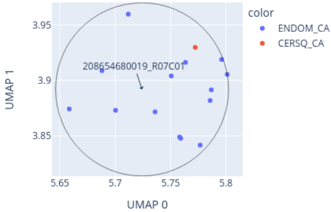
Close-up of UMAP for 208654680019_R07C01 reference: AllIDATv2_20210804_HPAP_Sarc.xlsx (19967 cases), 0 CpGs
