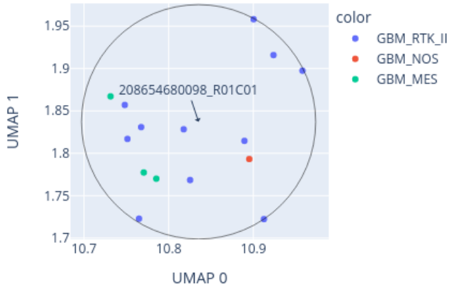
Close-up of UMAP for 208654680098_R01C01 reference: AllIDATv2_20210804_HPAP_Sarc.xlsx (19967 cases), 0 CpGs
