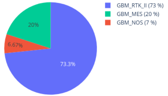
Neighbors in UMAP for 208654680098_R01C01 reference: AllIDATv2_20210804_HPAP_Sarc.xlsx (19967 cases), 0 CpGs
