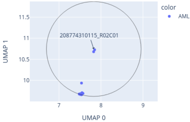
Close-up of UMAP for 208774310115_R02C01 reference: AllIDATv2_20210804_HPAP_Sarc.xlsx (19967 cases), 0 CpGs
