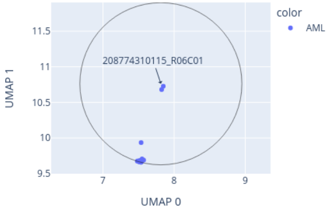
Close-up of UMAP for 208774310115_R06C01 reference: AllIDATv2_20210804_HPAP_Sarc.xlsx (19967 cases), 0 CpGs
