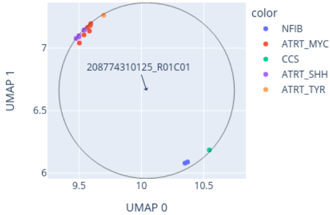
Close-up of UMAP for 208774310125_R01C01 reference: AllIDATv2_20210804_HPAP_Sarc.xlsx (19967 cases), 0 CpGs
