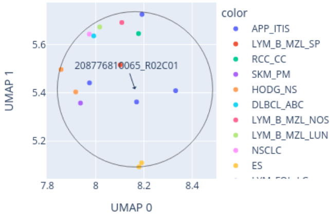
Close-up of UMAP for 208776810065_R02C01 reference: AllIDATv2_20210804_HPAP_Sarc.xlsx (19967 cases), 0 CpGs
