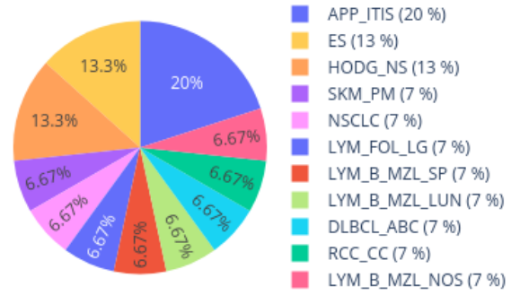
Neighbors in UMAP for 208776810065_R02C01 reference: AllIDATv2_20210804_HPAP_Sarc.xlsx (19967 cases), 0 CpGs
