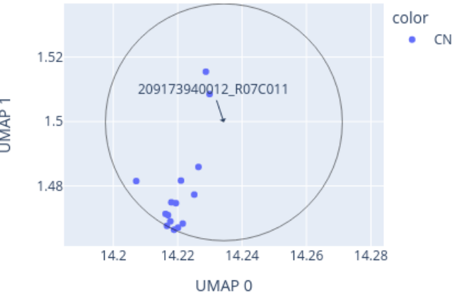
Close-up of UMAP for 209173940012_R07C011 reference: AllIDATv2_20210804_HPAP_Sarc.xlsx (19967 cases), 0 CpGs
