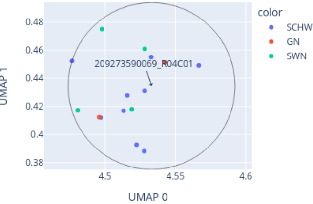
Close-up of UMAP for 209273590069_R04C01 reference: AllIDATv2_20210804_HPAP_Sarc.xlsx (19967 cases), 0 CpGs
