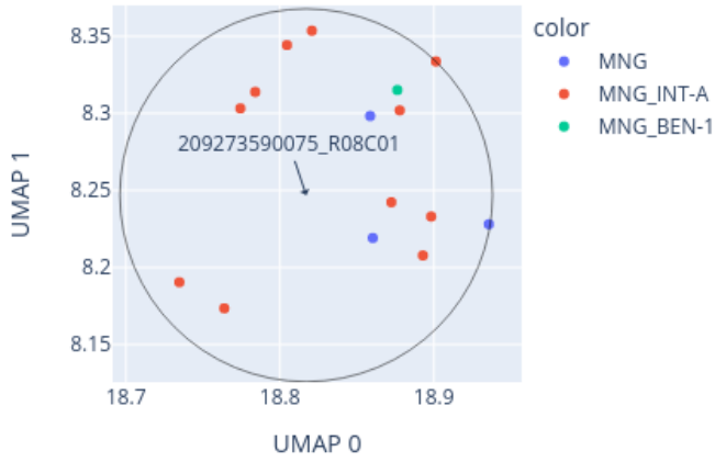
Close-up of UMAP for 209273590075_R08C01 reference: AllIDATv2_20210804_HPAP_Sarc.xlsx (19967 cases), 0 CpGs
