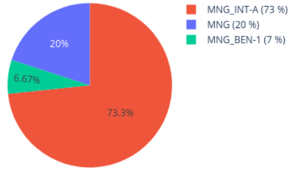
Neighbors in UMAP for 209273590075_R08C01 reference: AllIDATv2_20210804_HPAP_Sarc.xlsx (19967 cases), 0 CpGs
