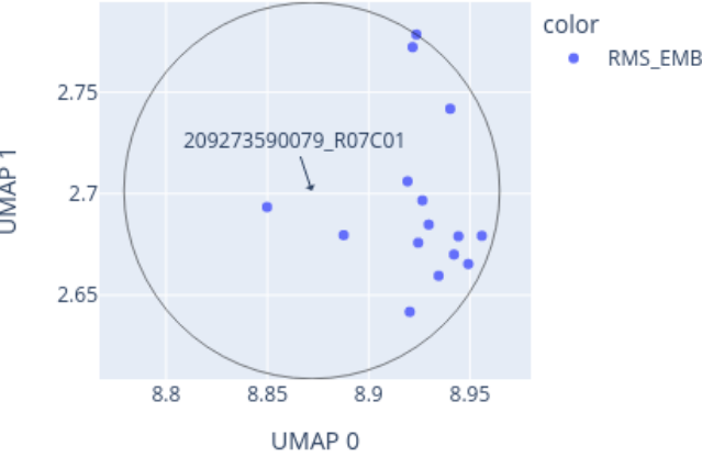
Close-up of UMAP for 209273590079_R07C01 reference: AllIDATv2_20210804_HPAP_Sarc.xlsx (19967 cases), 0 CpGs
