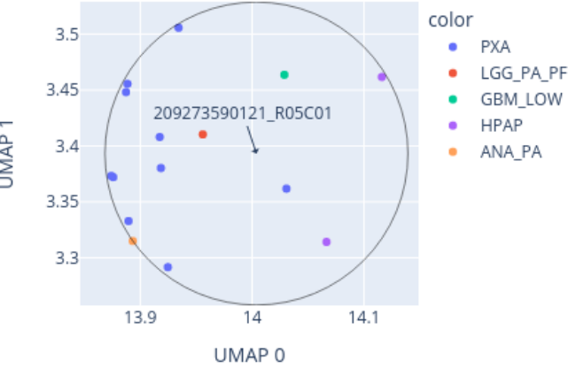
Close-up of UMAP for 209273590121_R05C01 reference: AllIDATv2_20210804_HPAP_Sarc.xlsx (19967 cases), 0 CpGs
