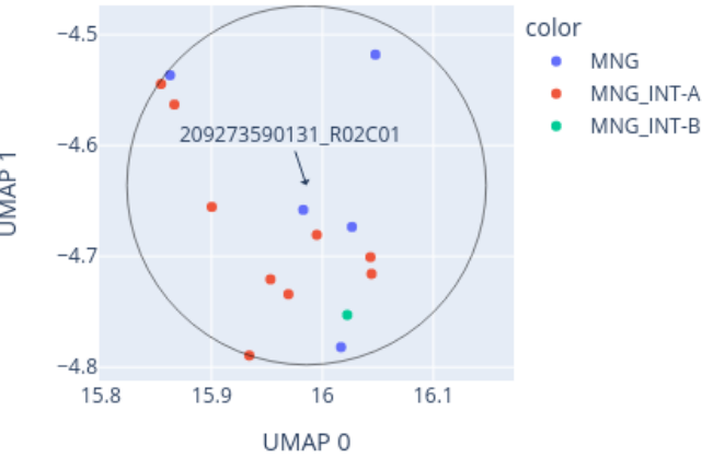
Close-up of UMAP for 209273590131_R02C01 reference: AllIDATv2_20210804_HPAP_Sarc.xlsx (19967 cases), 0 CpGs
