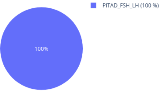
Neighbors in UMAP for 209273590168_R06C01 reference: AllIDATv2_20210804_HPAP_Sarc.xlsx (19967 cases), 0 CpGs
