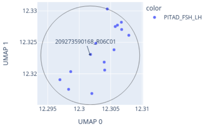
Close-up of UMAP for 209273590168_R06C01 reference: AllIDATv2_20210804_HPAP_Sarc.xlsx (19967 cases), 0 CpGs
