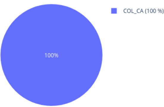
Neighbors in UMAP for 209274200075_R03C01 reference: AllIDATv2_20210804_HPAP_Sarc.xlsx (19967 cases), 0 CpGs
