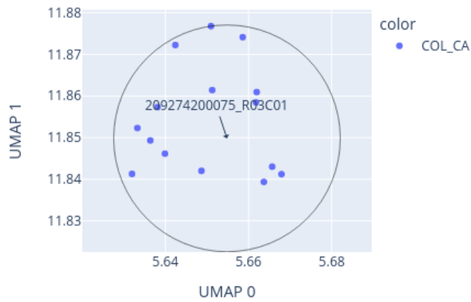
Close-up of UMAP for 209274200075_R03C01 reference: AllIDATv2_20210804_HPAP_Sarc.xlsx (19967 cases), 0 CpGs
