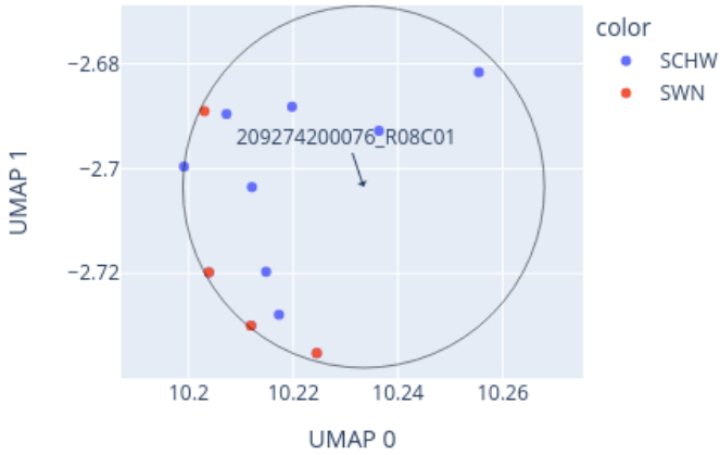
Close-up of UMAP for 209274200076_R08C01 reference: AllIDATv2_20210804_HPAP_Sarc.xlsx (19967 cases), 0 CpGs
