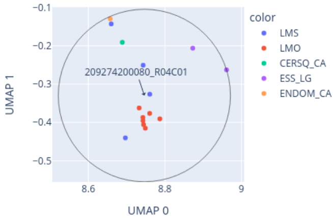
Close-up of UMAP for 209274200080_R04C01 reference: AllIDATv2_20210804_HPAP_Sarc.xlsx (19967 cases), 0 CpGs
