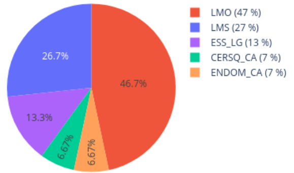
Neighbors in UMAP for 209274200080_R04C01 reference: AllIDATv2_20210804_HPAP_Sarc.xlsx (19967 cases), 0 CpGs
