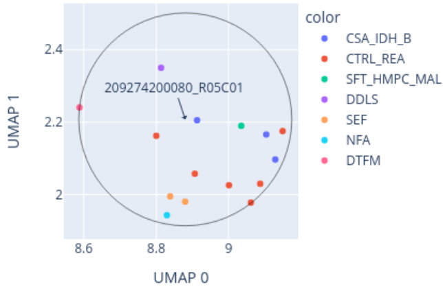
Close-up of UMAP for 209274200080_R05C01 reference: AllIDATv2_20210804_HPAP_Sarc.xlsx (19967 cases), 0 CpGs
