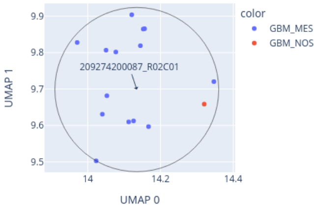
Close-up of UMAP for 209274200087_R02C01 reference: AllIDATv2_20210804_HPAP_Sarc.xlsx (19967 cases), 0 CpGs
