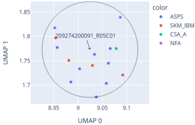
Close-up of UMAP for 209274200091_R05C01 reference: AllIDATv2_20210804_HPAP_Sarc.xlsx (19967 cases), 0 CpGs
