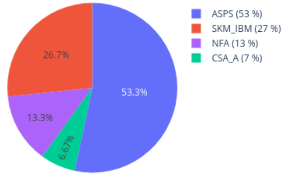
Neighbors in UMAP for 209274200091_R05C01 reference: AllIDATv2_20210804_HPAP_Sarc.xlsx (19967 cases), 0 CpGs
