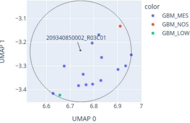
Close-up of UMAP for 209340850002_R03C01 reference: AllIDATv2_20210804_HPAP_Sarc.xlsx (19967 cases), 0 CpGs
