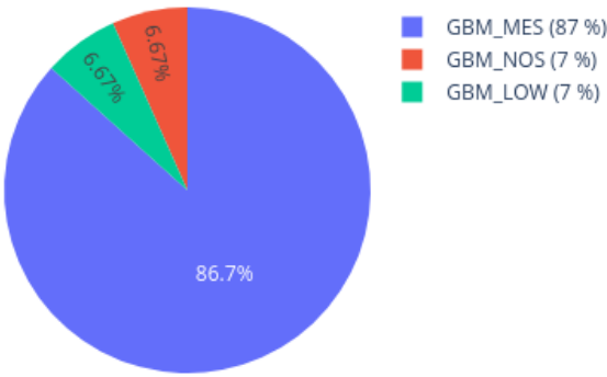
Neighbors in UMAP for 209340850002_R03C01 reference: AllIDATv2_20210804_HPAP_Sarc.xlsx (19967 cases), 0 CpGs
