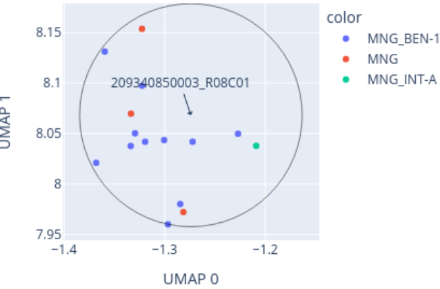
Close-up of UMAP for 209340850003_R08C01 reference: AllIDATv2_20210804_HPAP_Sarc.xlsx (19967 cases), 0 CpGs
