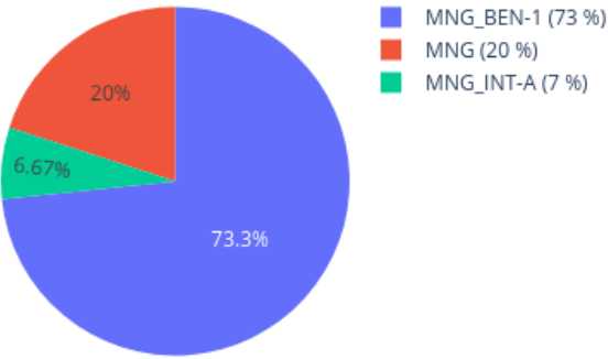
Neighbors in UMAP for 209340850003_R08C01 reference: AllIDATv2_20210804_HPAP_Sarc.xlsx (19967 cases), 0 CpGs
