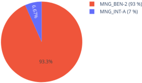
Neighbors in UMAP for 209340850028_R07C01 reference: AllIDATv2_20210804_HPAP_Sarc.xlsx (19967 cases), 0 CpGs
