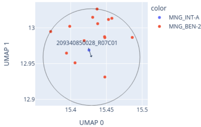
Close-up of UMAP for 209340850028_R07C01 reference: AllIDATv2_20210804_HPAP_Sarc.xlsx (19967 cases), 0 CpGs
