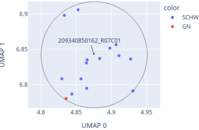
Close-up of UMAP for 209340850162_R07C01 reference: AllIDATv2_20210804_HPAP_Sarc.xlsx (19967 cases), 0 CpGs
