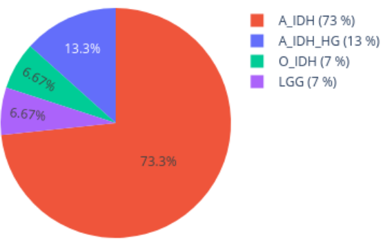
Neighbors in UMAP for 209340870007_R04C01 reference: AllIDATv2_20210804_HPAP_Sarc.xlsx (19967 cases), 0 CpGs
