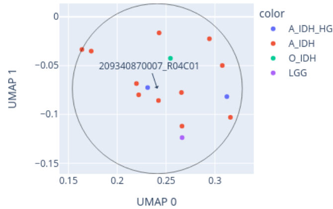
Close-up of UMAP for 209340870007_R04C01 reference: AllIDATv2_20210804_HPAP_Sarc.xlsx (19967 cases), 0 CpGs
