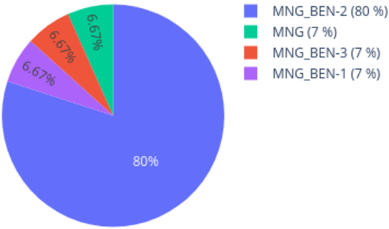
Neighbors in UMAP for 209340870007_R06C01 reference: AllIDATv2_20210804_HPAP_Sarc.xlsx (19967 cases), 0 CpGs
