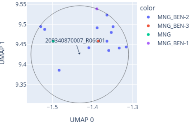
Close-up of UMAP for 209340870007_R06C01 reference: AllIDATv2_20210804_HPAP_Sarc.xlsx (19967 cases), 0 CpGs
