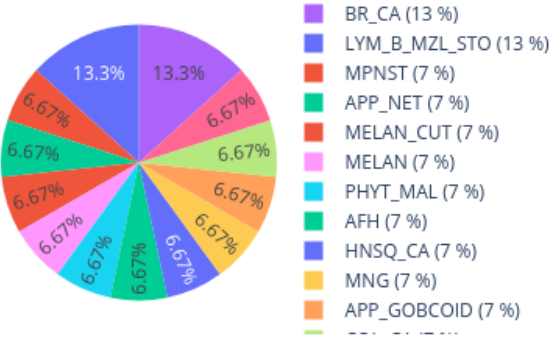
Neighbors in UMAP for 209340870107_R05C01 reference: AllIDatv2_20210804_HPAP_Sarc.xlsx (19967 cases), 0 CpGs
