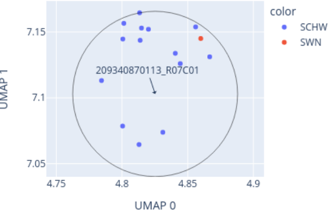
Close-up of UMAP for 209340870113_R07C01 reference: AllIDATv2_20210804_HPAP_Sarc.xlsx (19967 cases), 0 CpGs
