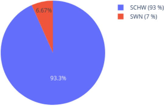
Neighbors in UMAP for 209340870113_R07C01 reference: AllIDATv2_20210804_HPAP_Sarc.xlsx (19967 cases), 0 CpGs
