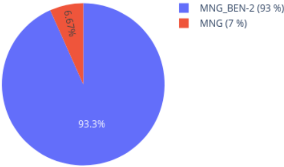
Neighbors in UMAP for 209403880129_R05C01 reference: AllIDATv2_20210804_HPAP_Sarc.xlsx (19967 cases), 0 CpGs
