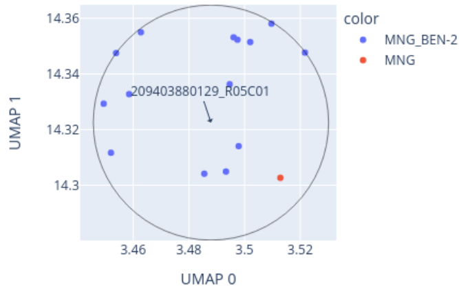
Close-up of UMAP for 209403880129_R05C01 reference: AllIDATv2_20210804_HPAP_Sarc.xlsx (19967 cases), 0 CpGs
